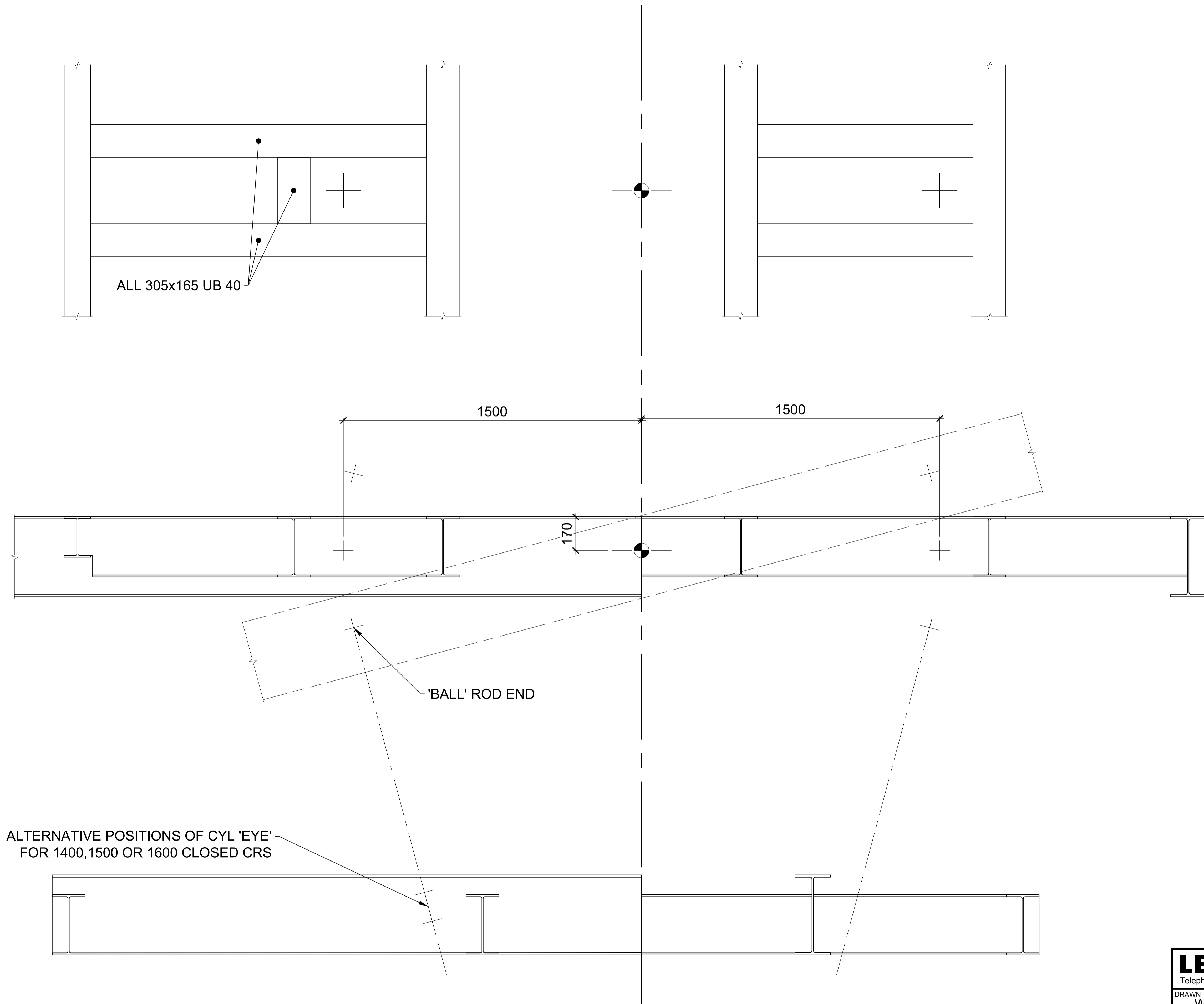
HALF SECTION OF LENGTH (PITCH)
